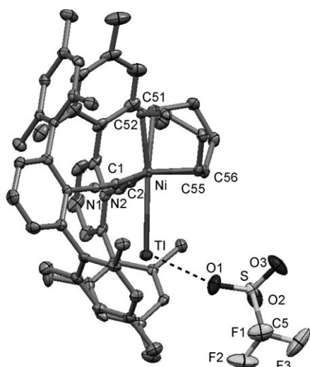
Figure 1. Molecular structure of [\text{TiNi}(\text{cod})(\text{CNAr}^{\text{Mes}_2})_2]\text{OTf} . Thermal ellipsoids are set at 50% probability. Hydrogen atoms are omitted for clarity.
