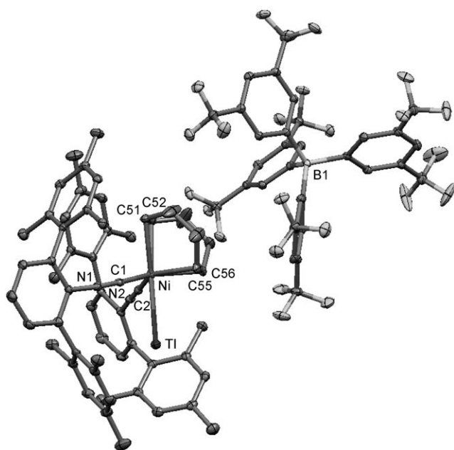
Figure 2. Molecular structure of [\text{TiNi}(\text{cod})(\text{CNAr}^{\text{Mes}_2})_2]\text{BARF}_4 . Thermal ellipsoids are set at 50% probability. Hydrogen atoms are omitted for clarity.
